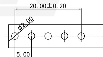
RECOMMENDED PCB LAYOUT TOP VIEW (.XX ± 0.05)
